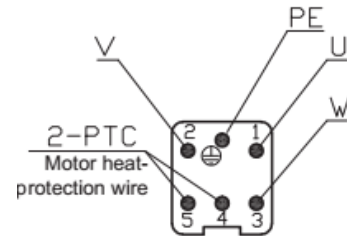
Wiring description diagram
